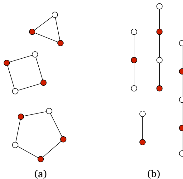
Figure 12.7: Examples for minimum vertex covers of cycles (a) and paths (b).
