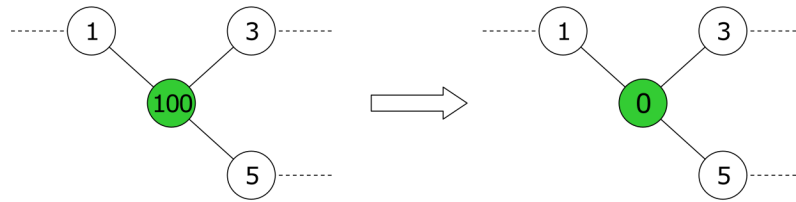
Figure 1.8: Vertex 100 receives the lowest possible color.
